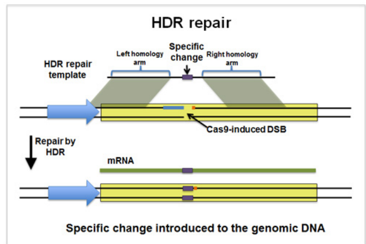
Figure 1: The HDR repair template contains a specific change in the middle of sequences homologous to the genomic DNA. After a Cas9-induced DSB, the break is repaired by HDR which introduces the specific change into the genomic DNA.
