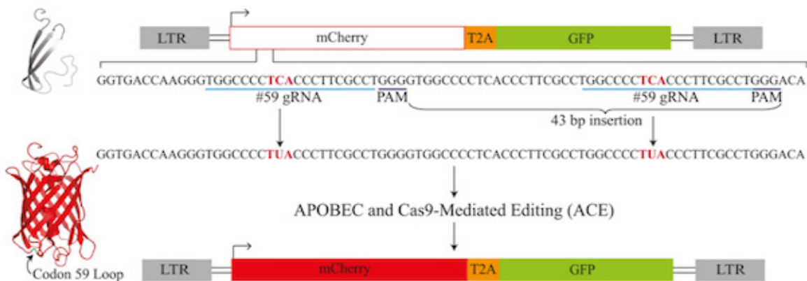
Figure 1: APOBEC- and Cas9-mediated editing (ACE) reporter in action. Image from St. Martin et al., 2018.
