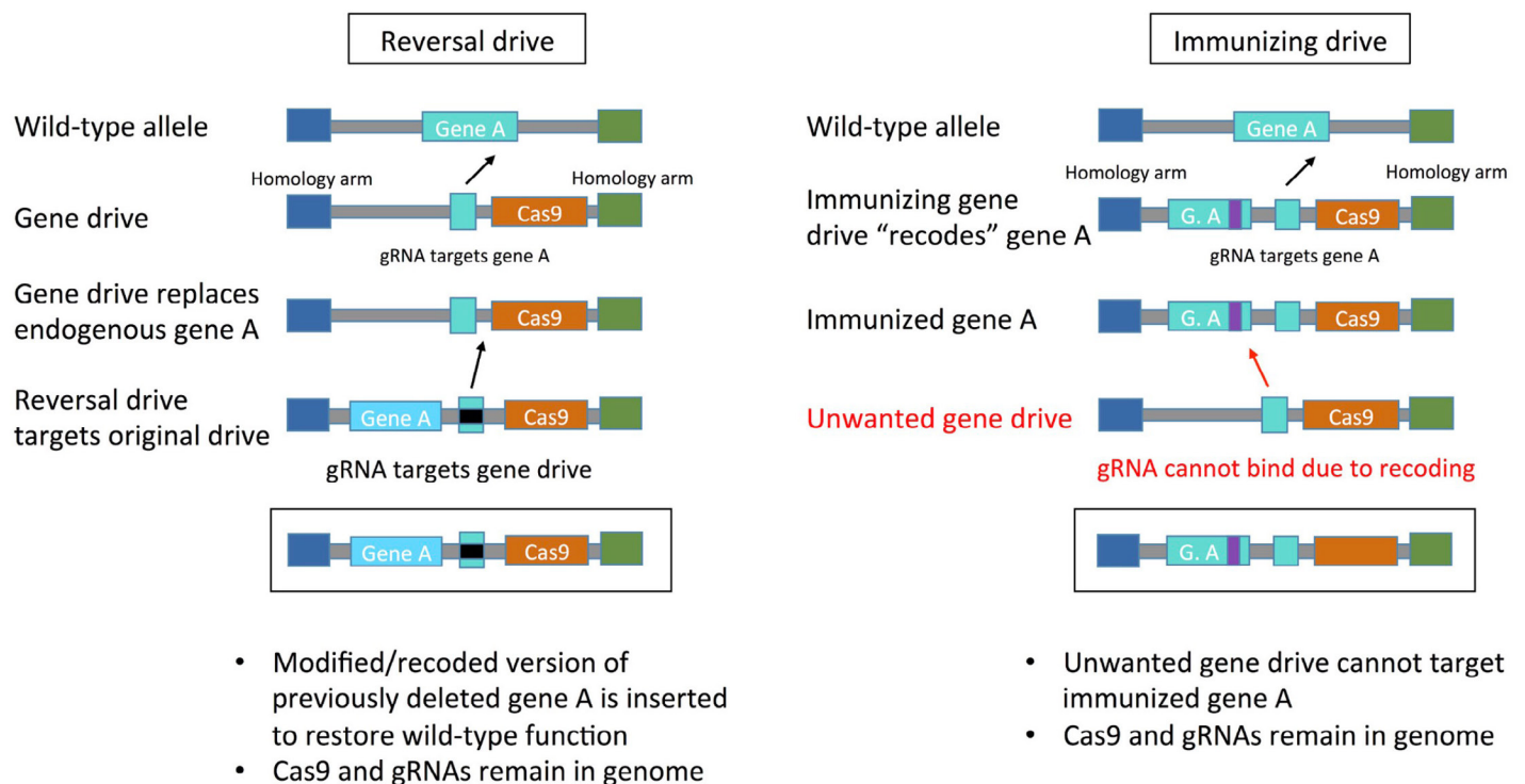
Figure 2: Reversal and immunizing drives. Reversal drives “reverse” previous gene drives by reintroducing previously edited/deleted genes. Immunizing drives modify a gene of interest to prevent other gene drives from targeting it. Figure adapted from Esvelt et al.
