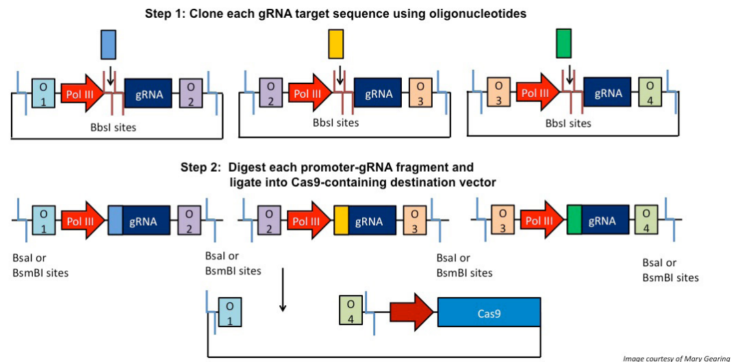
Figure 2: gRNA target sequences are cloned into various plasmids using oligonucleotides. These plasmids contain Type IIS restriction sites that flank the promoter-gRNA constructs. When these plasmids are digested, unique overhangs (here, O1-4) adjacent to the cut sites “link” fragments together and drive ordered assembly into a Cas9-containing destination vector. Note: depending on which method you use, the procedure will vary slightly.
