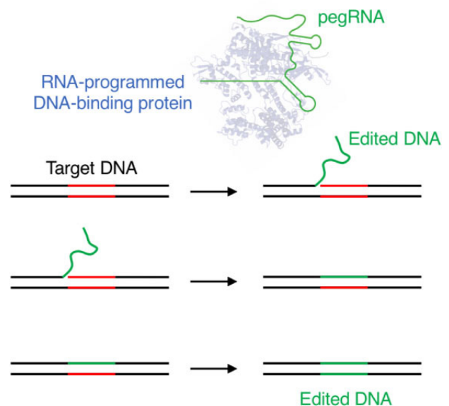
Figure 1: The prime editing guide RNA (pegRNA) specifies the target site and contains the edit. After Cas9 nicking, the reverse transcriptase domain uses pegRNA to reverse transcribe the edit. The edited strand replaces the original DNA strand. Resolution of the heteroduplex to favor copying the edit onto the unedited strand completes the process. Image from David Liu with permission.
