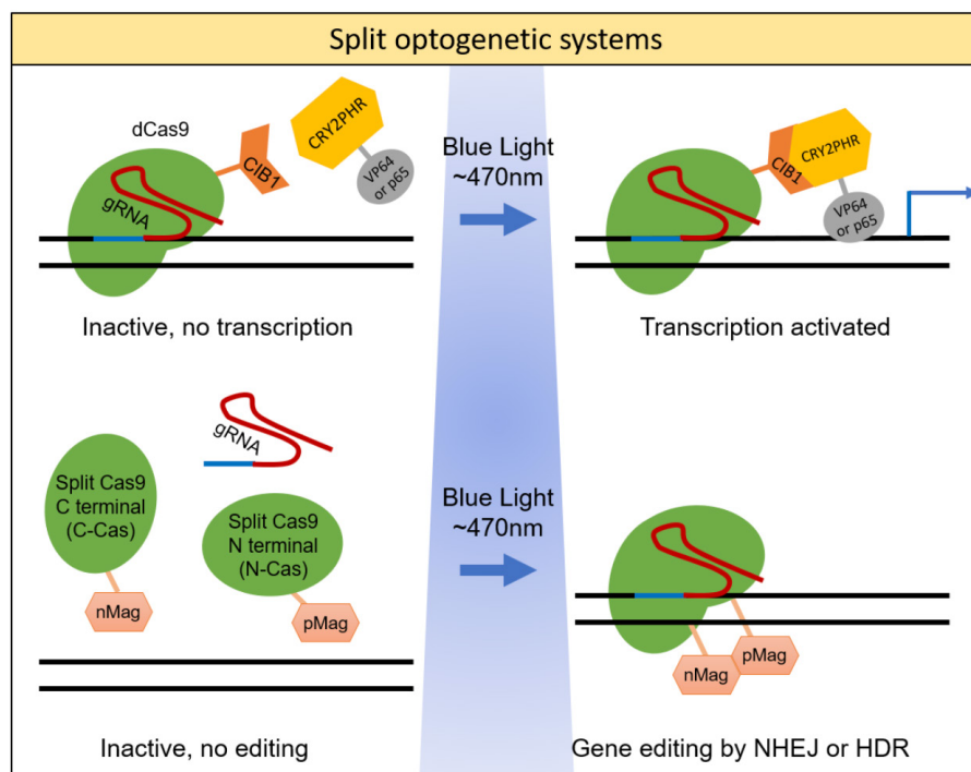
Figure 1: These split optogenetic system is activated by blue light to cause transcriptional activation or editing at target locus.
