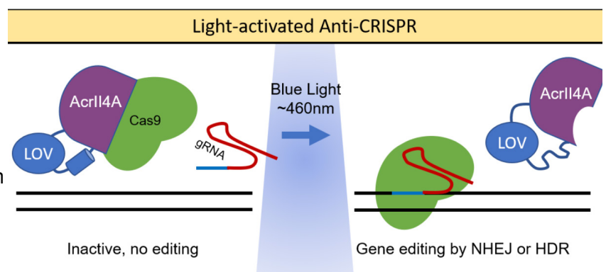
Figure 3: Anti-CRISPR activity controlled with blue light. With blue light, the anti-CRISPR activity is alleviated.
