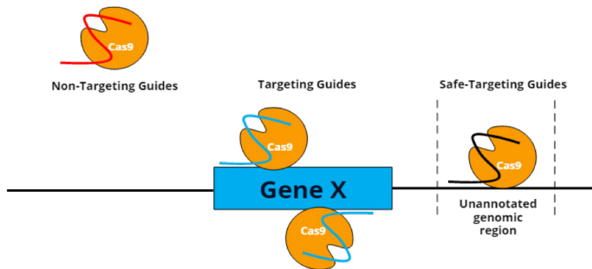
Figure 2: Non-targeting vs. safe-targeting guides. The genome-wide CRISPR screen presented in Morgens et al. contains three types of guides: 1) targeting guides (blue), which target all protein-coding genes present in the genome; 2) non-targeting guides which target no sequence in the genome. Non-targeting guides (red) are commonly used as negative controls for genome-wide CRISPR screens; and 3) safe-targeting guides which target genomic sites with no annotated function.
