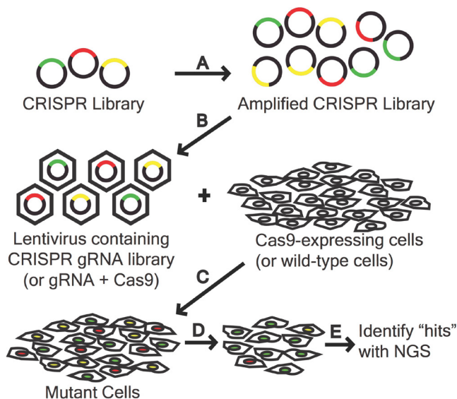
Figure 1: The CRISPR library must be amplified to be used to generate lentivirus. Cas9-expressing cells or wild-type cells are treated with lentivirus containing the gRNA library or gRNA library with Cas9 to generate mutant cells, respectively. Mutant cells are screened and hits are identified using NGS.
