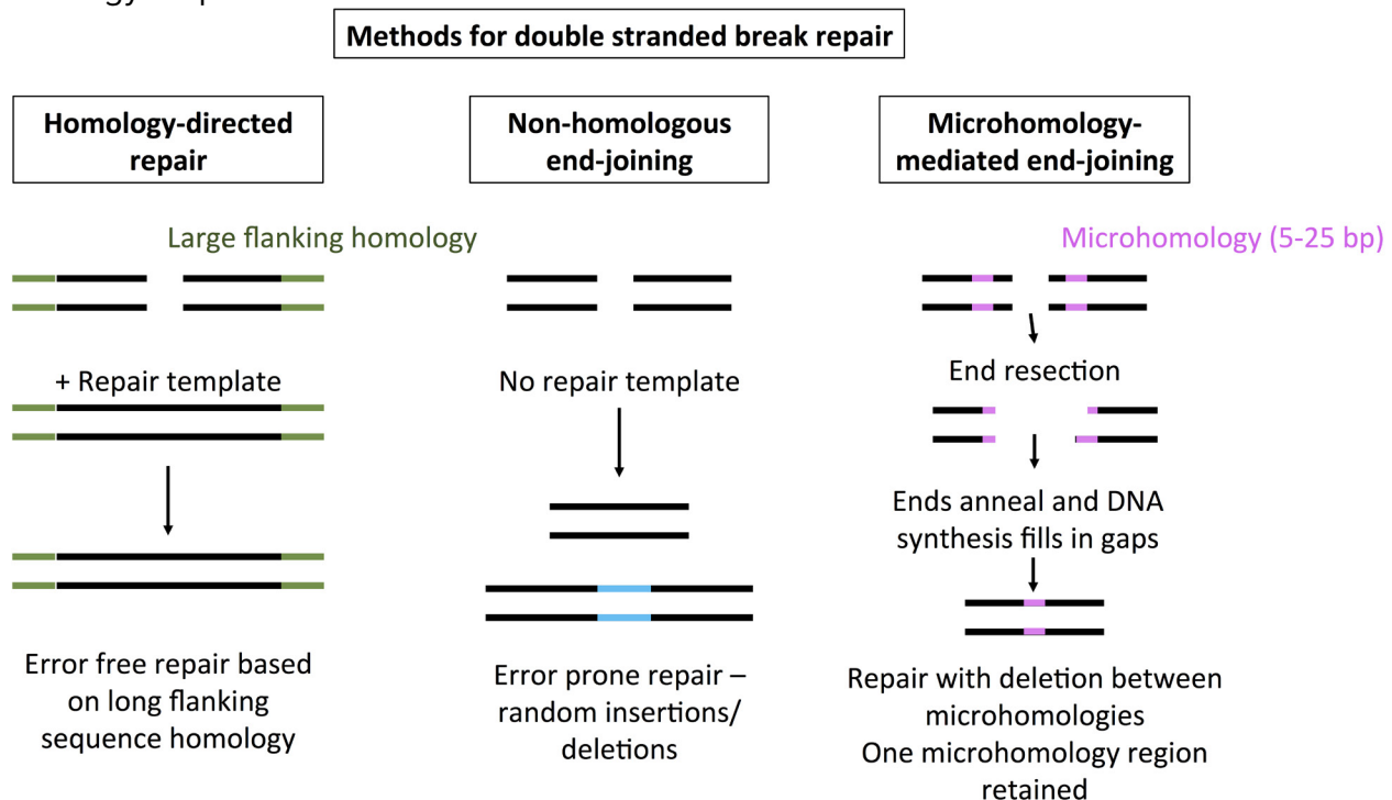
Figure 1: Three methods for double stranded break repair.
