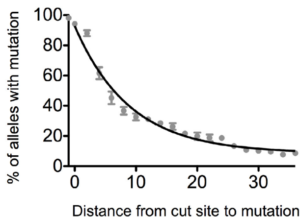
Figure 2: Relationship between cut site to mutation distance and editing efficiency.
