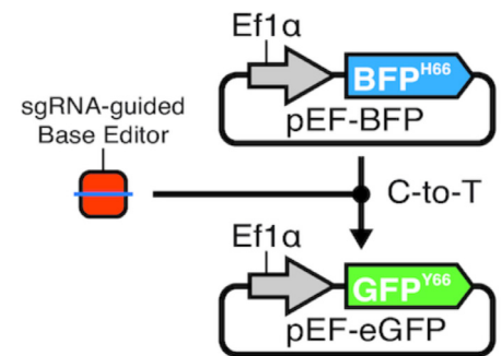
Figure 2: Targeting pEF-BFP with a cytidine deaminase base editor results in shift in emission spectra from BFP to GFP. Image from Standage-Beier et al., 2019.
