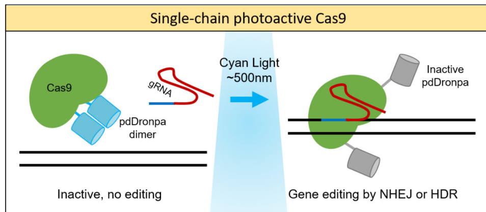
Figure 2: A fusion protein of Cas9 with photo-dissociable dimeric GFP responds to cyan light. Without light, the dimer blocks Cas9. With light, Cas9 can bind DNA.
