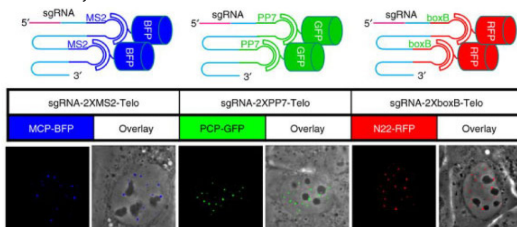
Figure 1: CRISPRainbow labeling. Two MS2, PP7, or boxB sequences inserted into the sgRNA generates blue, green, or red colors for labeling. A combination of MS2, PP7, or boxB sequences in the same sgRNA will generate additional colors. Image from Ma et al., 2016 with permission.
